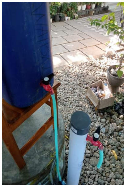
Alat filtrasi downflow
