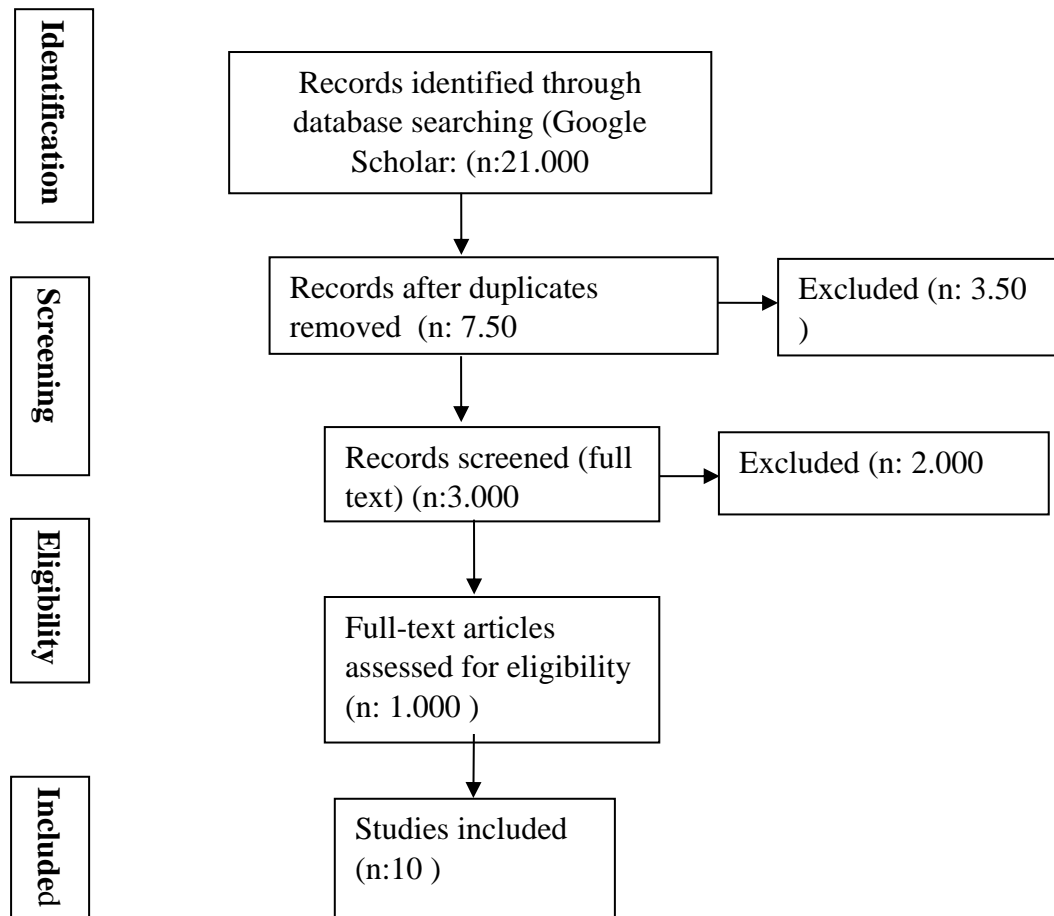
Gambar 3.5 Prisma Chart
